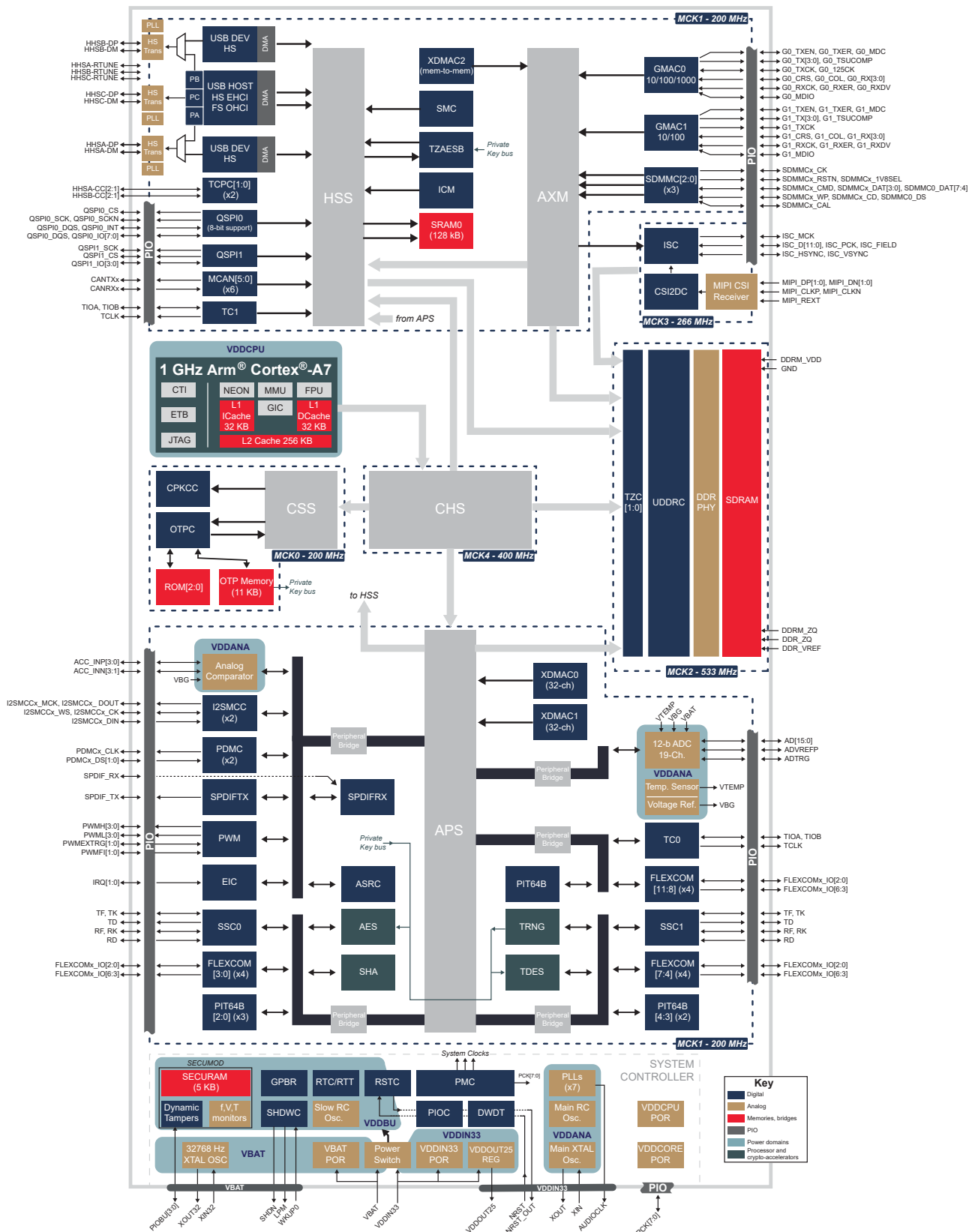
Figure 7-1. SAMA7G5 Series SiP Block Diagram
